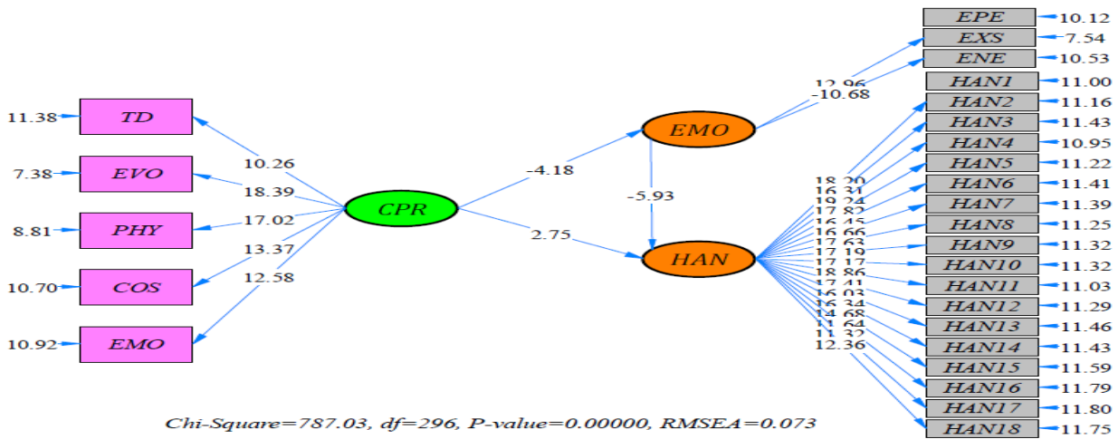
Significance Values of the Structural Model
